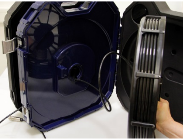
Fig. 67: Removing the viper with the connection cable from the case.
